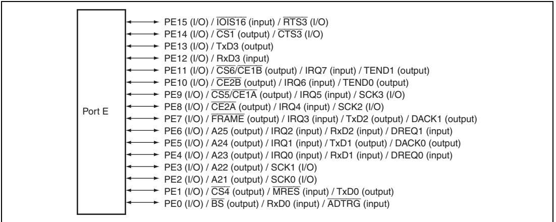
Figure 30.5 Port E
