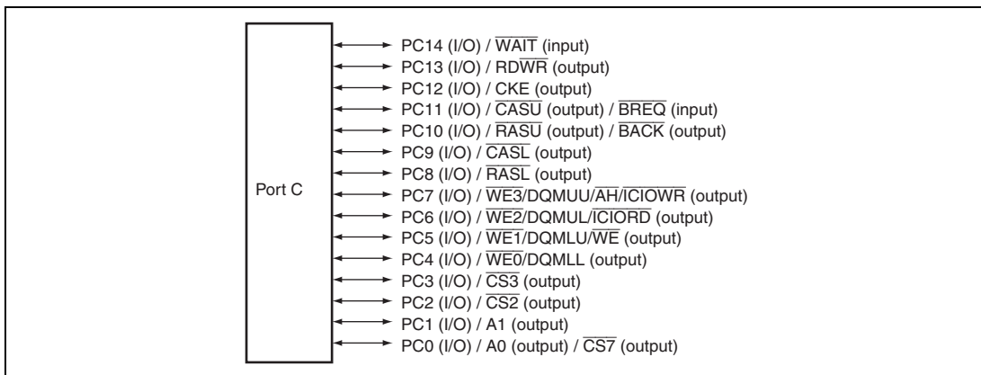
Figure 30.3 Port C
