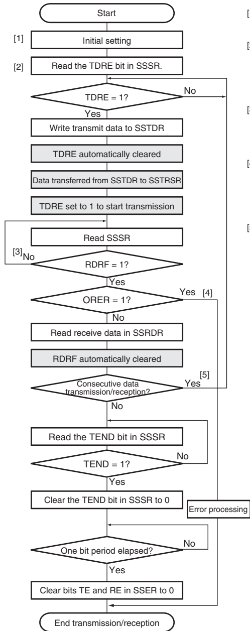
Figure 16.17 Flowchart Example of Simultaneous Transmission/Reception (Clock Synchronous Communication Mode)
