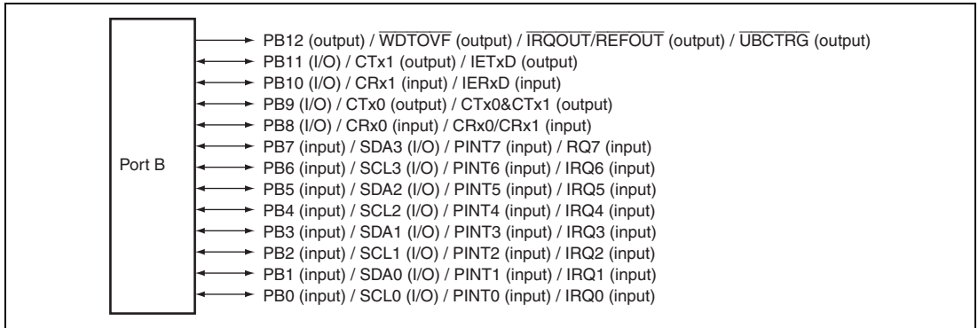
Figure 30.2 Port B
