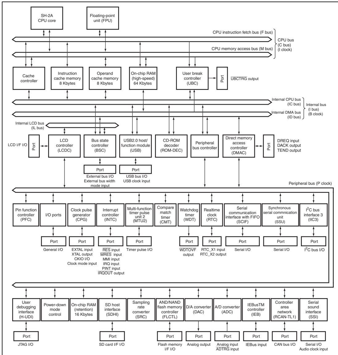
Figure 1.1 Block Diagram
